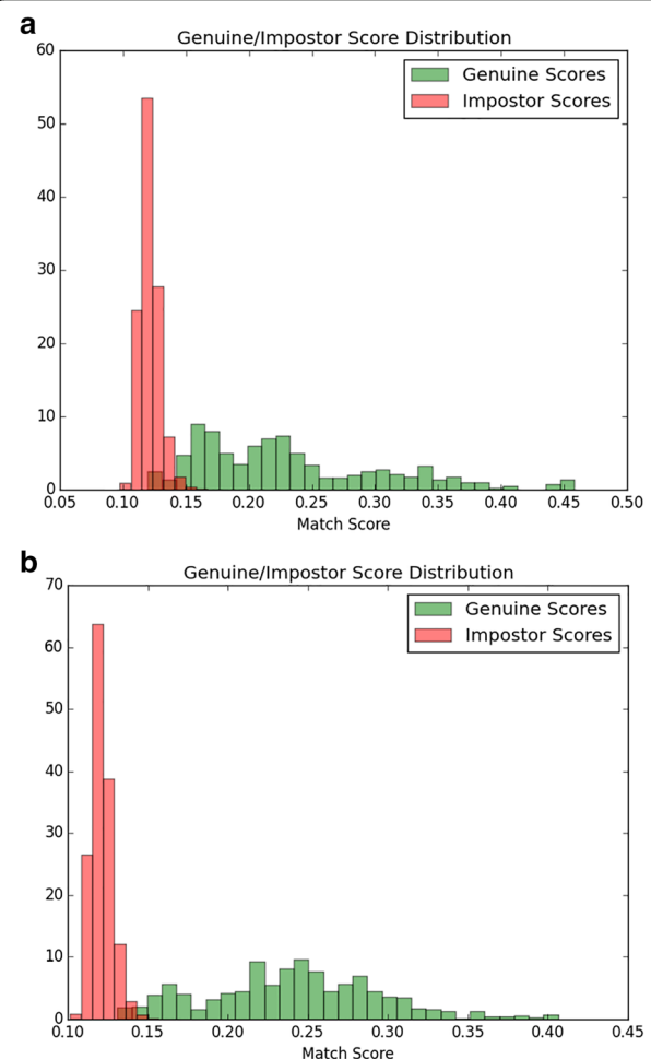
Fig. 11 Histograms of genuine (correct match) vs. impostor (incorrect match) scores. a Results with only one query image (4,265 genuine, 831,583 impostor). b Results with 2 query images (4,317 genuine, 841,743 impostor)
