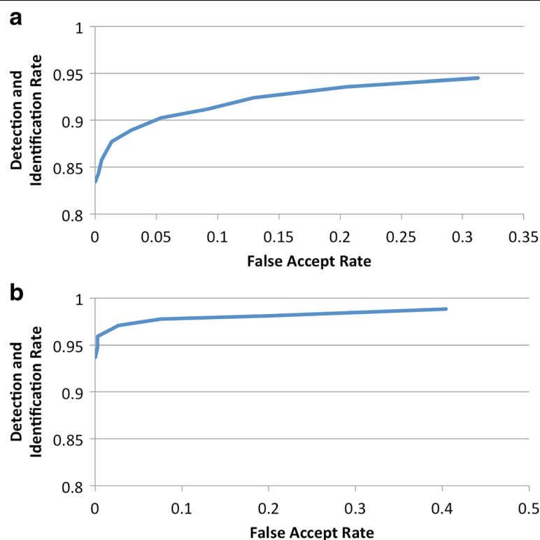
Fig. 12 DIR curve for open-set matching with 2 query images. Plots show the proportion of in-gallery lemurs that were correctly identified (DIR) at (a) rank 1 and (b) rank 5 versus the proportion of novel individuals that were matched to a gallery individual (FAR)
